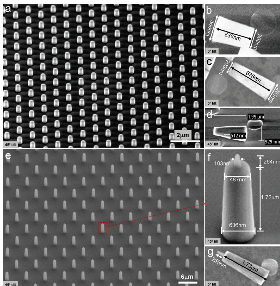
Figure 3. SEM images of fabricated quartz particles. (a) Fabricated quartz cylinders (nominal top diameter: 300-nm) arranged in a hexagonal array pattern on the wafer. (b) A single quartz cylinder after microtome shaving off the wafer (from the same wafer as in panel a). The microtome shaving consistently produces an evenly cut surface at the base of the quartz cylinder, and the cross section of the cut surface demonstrates a round shape at the cylinder's base. (c) A cylinder with a smaller diameter (nominal top diameter: 200 nm) and a higher aspect ratio. (d) A larger cylinder (nominal top diameter: 500 nm) fabricated with a slightly more conical shape. (e–g) Larger cylinders (nominal top diameter: 500 nm) with centered protrusions. (e) Demonstration that the centered protrusions were fabricated consistently on all cylinders in the patterned area. (f) A typical feature size of the centered-protrusion cylinder. (g) A single cylinder with a centered protrusion following microtome shaving. In all panels, the tilt angle of the wafer surface for SEM imaging is indicated in the bottom-left corner.
